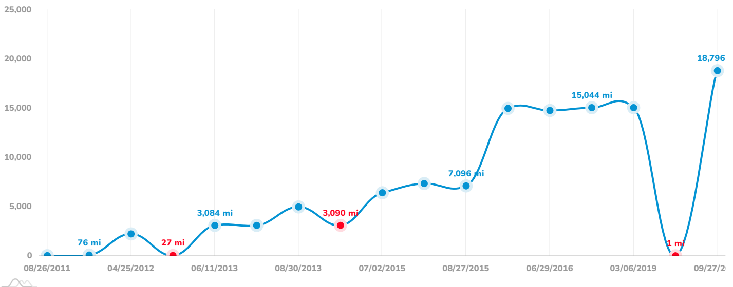
Mileage/Year Dependence
