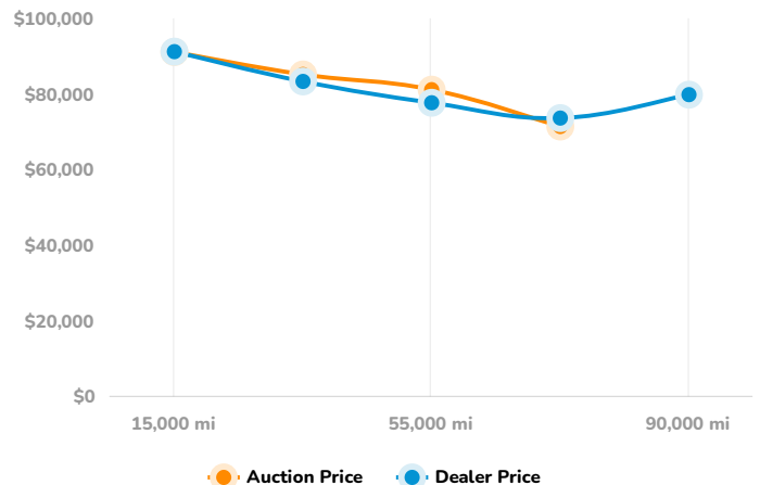
Price/Mileage Dependence
