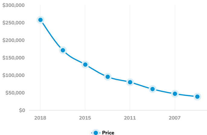
Price/Year Dependence
